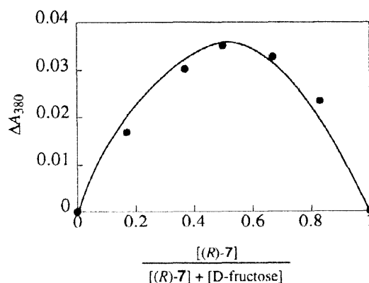
Fig. 4 Job plot for the complex formation from ( R )- 7 and D-fructose: 25 °C, water (pH 9.5 with 50 mmol dm -3 carbonate buffer)-methanol = 1:1 (v/v).
