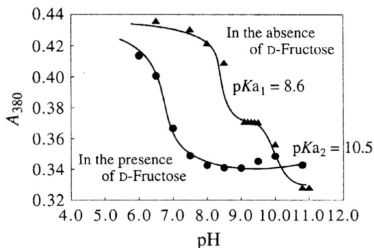
Fig. 3 Plots of A_{380} vs. pH in the absence and the presence of D-fructose
