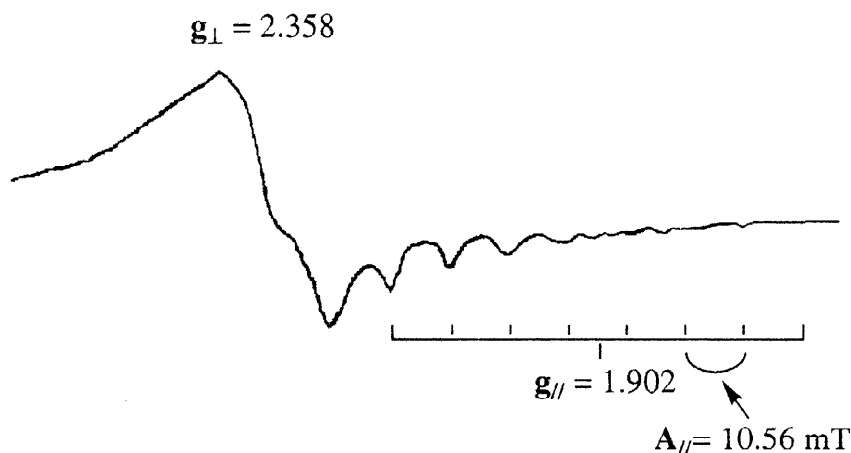
Fig. 1 ESR spectrum of (R)-7 ( 6.0 \times 10^{-4} \text{ mol dm}^{-3} ) in DMSO at 25^\circ\text{C}
