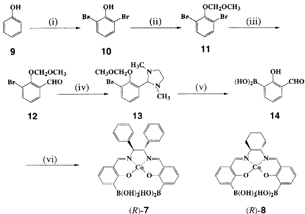
Scheme 1 (i) t -BuNH 2 , Br 2 , toluene, (ii) NaH, CH 3 OCH 2 Cl, THF, (iii) n -BuLi, DMF, THF, (iv) CH 3 NHCH 2 CH 2 NHCH 3 , toluene, (v) n -BuLi, B(OMe) 3 , THF, (vi) Co(OAc) 2 , ( R )-1,2-diphenylethylenediamine for ( R )- 7 and ( R )-1,2-diaminocyclohexane for ( R )- 8 , EtOH
