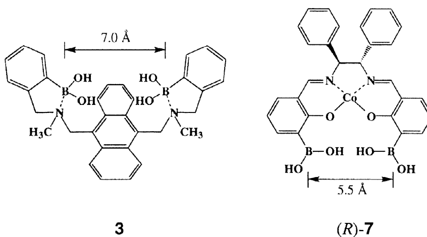
Fig. 8 Distance between two boronic acid groups of 3 and ( R )- 7
