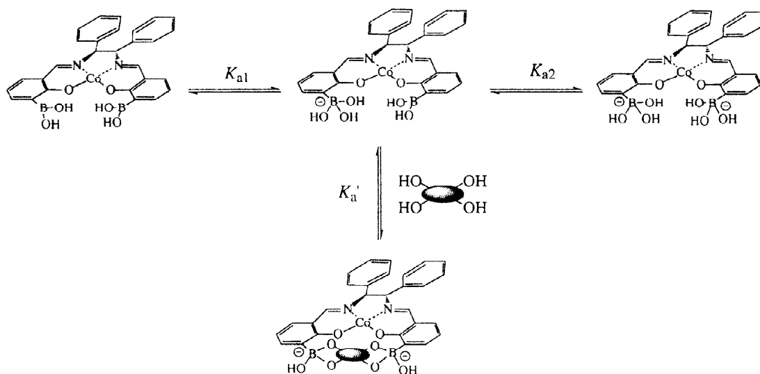
Scheme 2 Acid dissociation of ( R )-7 and complexation with D-fructose
