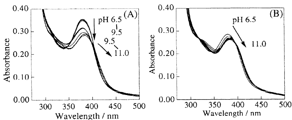
Fig. 5 pH dependence of the absorption spectra of ( R )- 8 ( 5.0 \times 10^{-5} mol dm -3 ) in the absence (A) and the presence of D-fructose (0.1 mol dm -3 ): 25 °C, water (50 mmol dm -3 buffer) - methanol = 1:1 (v/v).
