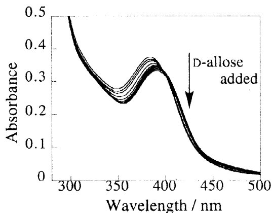
Fig. 6 Absorption spectral change in ( R )- 7 ( 5.0 \times 10^{-5} \text{ mol dm}^{-3} ) in the presence of D-allose ( 0 \sim 1.5 \times 10^{-2} \text{ mol dm}^{-3} ); the measurement conditions are recorded in the caption to Fig. 5.
