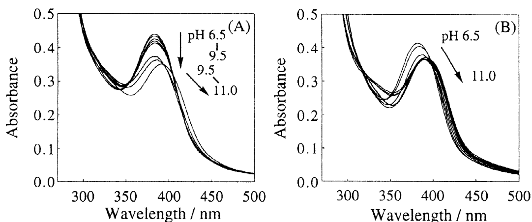
Fig. 2 pH dependence (6.5 - 11.0) of the absorption spectra of ( R )- 7 ( 5.0 \times 10^{-5} mol dm -3 ) in the absence (A) and the presence (B) of D-fructose ( 0.10 mol dm -3 ): 25 °C, water ( 50 mmol dm -3 buffer) - methanol = 1:1 (v/v)
